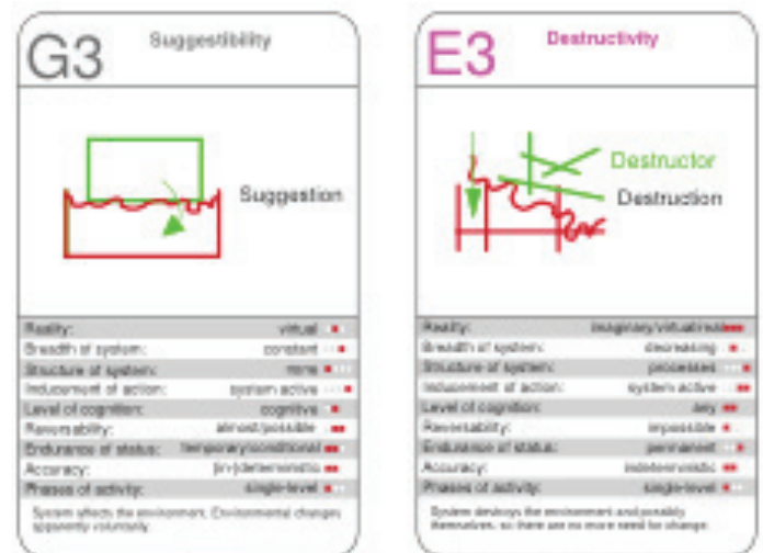
Figure 4. Strategy patterns
